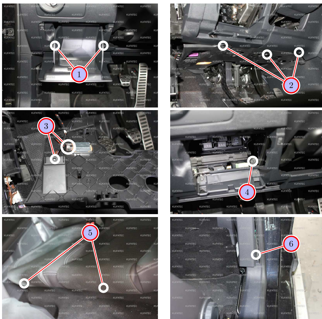
Figure 5: Removing lower trim of the instrument panel and oddments tray - pictures
