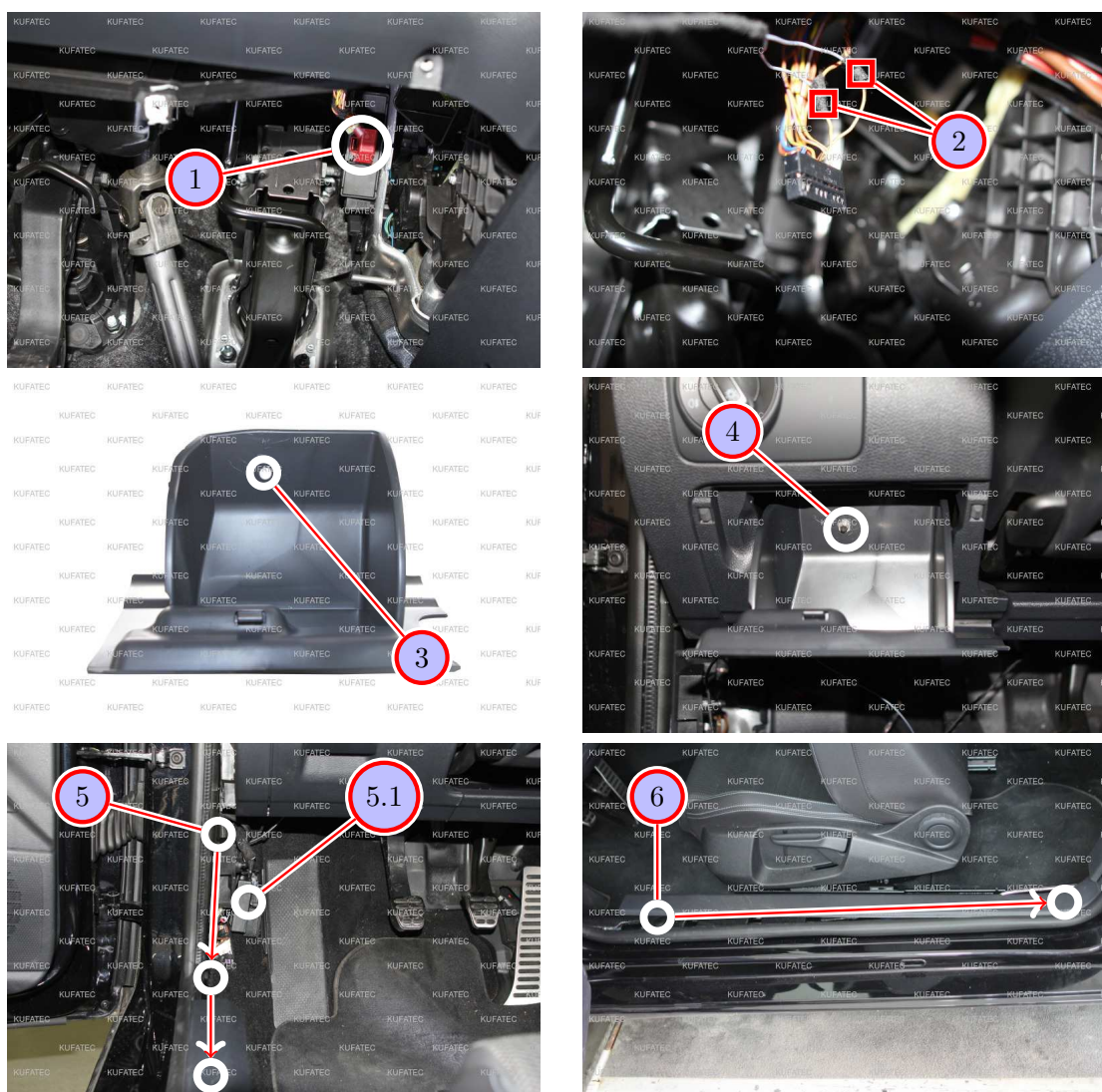
Figure 7: Connection CAN-Bus, installation pushbutton and cable routing - pictures
