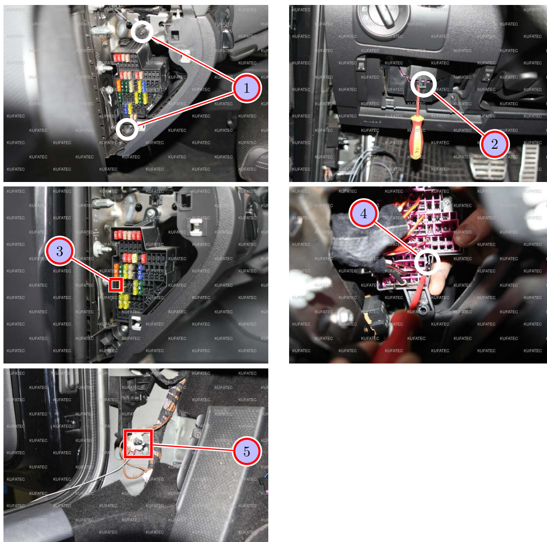
Figure 6: Connection ignition lead and ground - pictures
