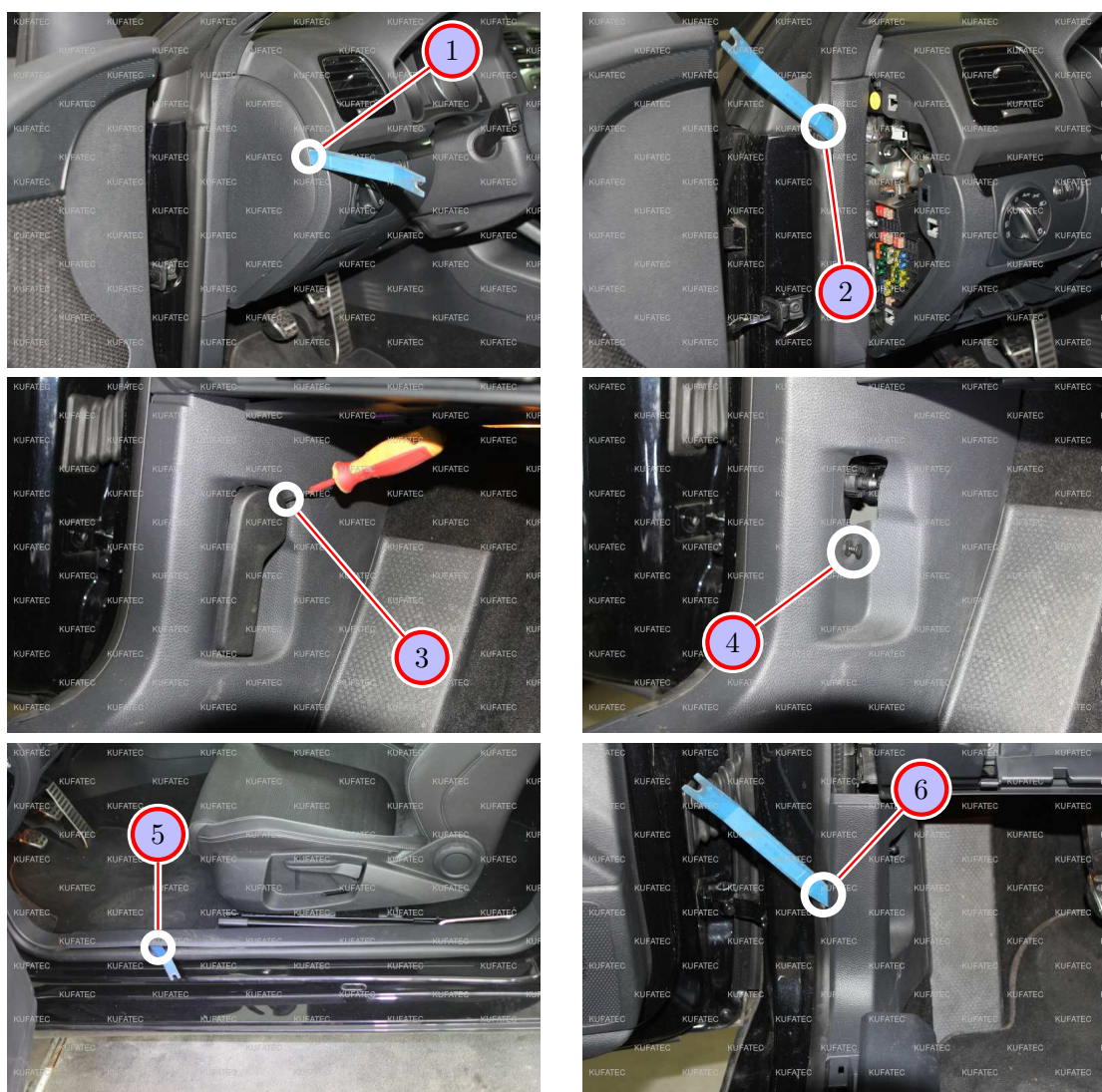
Figure 4: Removing trim panel and hood release - pictures
